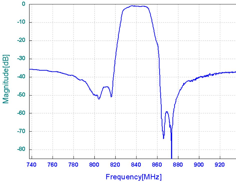
Frequency Response
